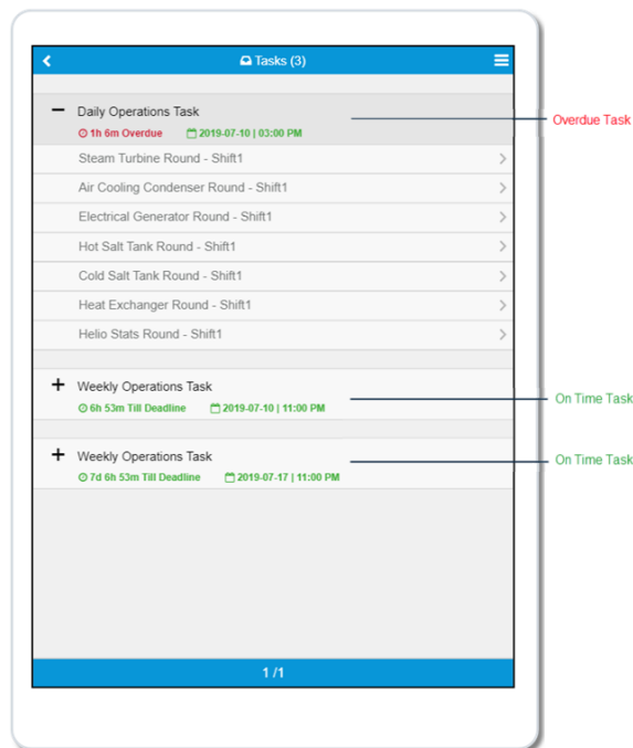
Figure 16 Tasks page
