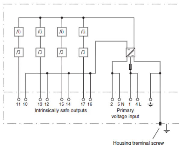
Figure 1. Connection Diagram
