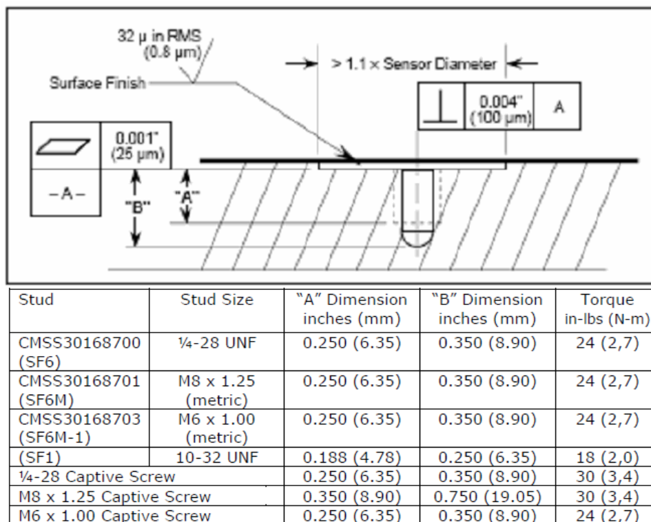
Figure 1. Surface preparation details
