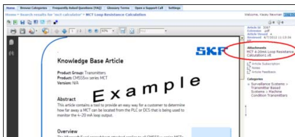
Figure 1. Attachments section
