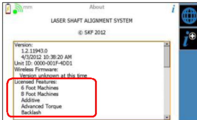
Figure 2. About menu
