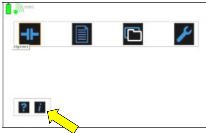
Figure 1. Home menu
