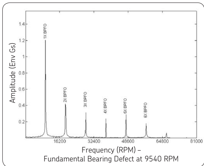
Example of an enveloped spectrum (outer race).
