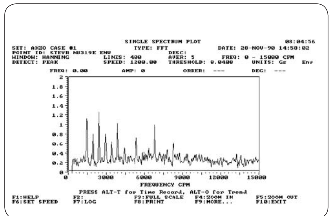
The enveloped spectrum of the previous velocity measurement, again peaks shown represent cage defect.
