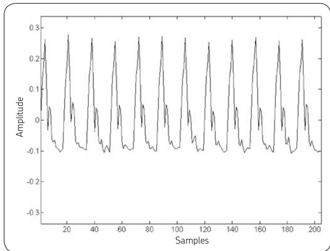
Example of an enveloped time waveform (outer race).
