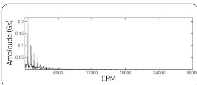
The same bearing's enveloped acceleration spectrum.
