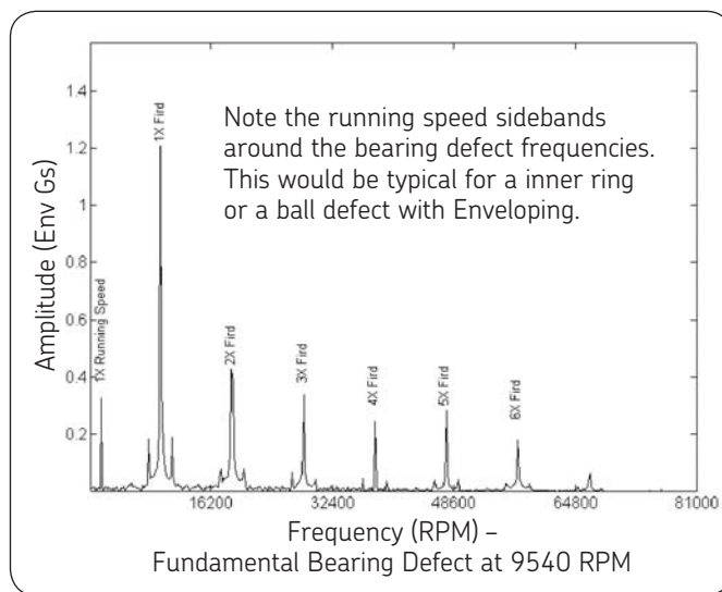
Example of an enveloped spectrum (outer race) for radial loaded bearings.
