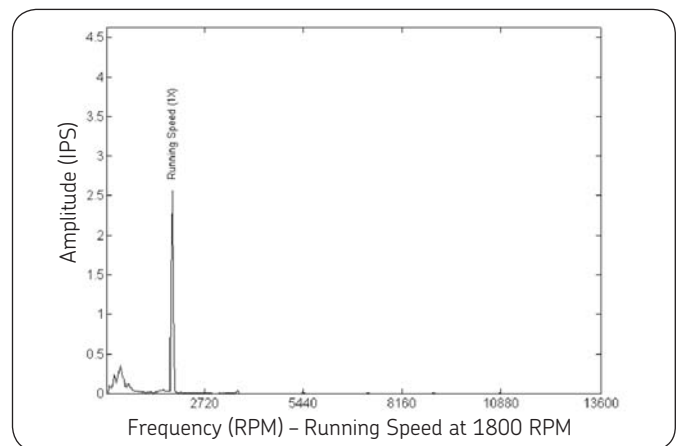
FFT spectrums showing imbalance.
