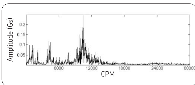
A spalled bearing's acceleration vibration spectrum.
